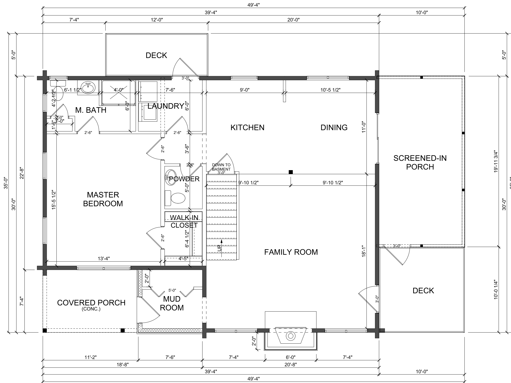
MAIN LEVEL FLOORPLAN SCALE: 1/4" = 1'-0"
